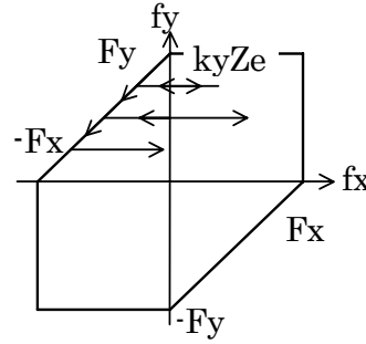
Fig.12 Tresca yield criterion
