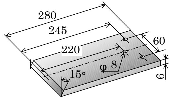
Fig.5 Size of specimen for butt-welding
