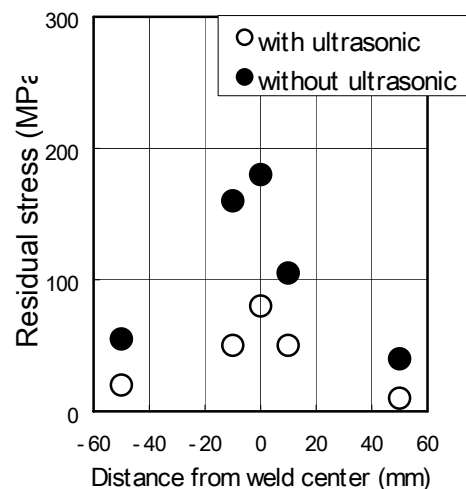
Fig.6 Residual stress of butt-welded specimen
