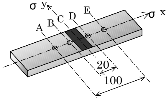
Fig.3 Measuring locations of residual stress
