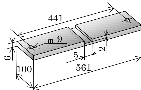
Fig.1 Size of specimen with groove
