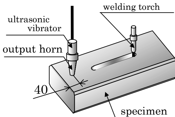
Fig.8 Experimental setup for welding of thick plate
