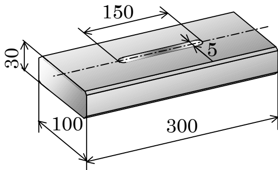
Fig.7 Size of thick plate
