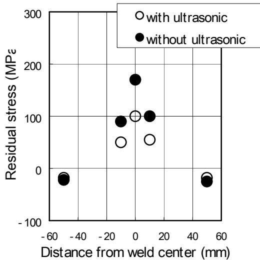
Fig.4 Residual stress of specimen with groove
