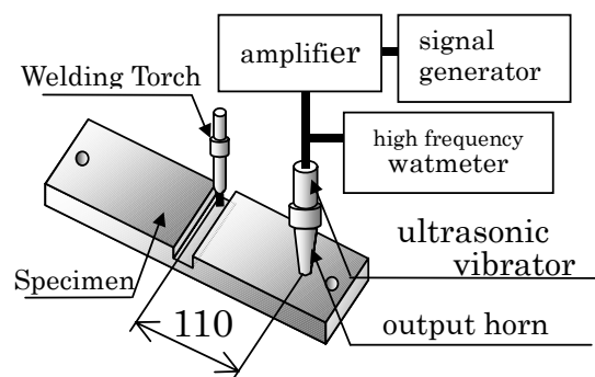
Fig.2 Experimental setup for butt-welding
