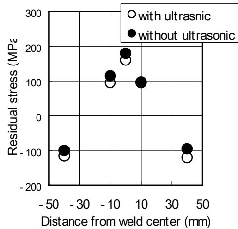
Fig.10 Residual stress of thick plate
