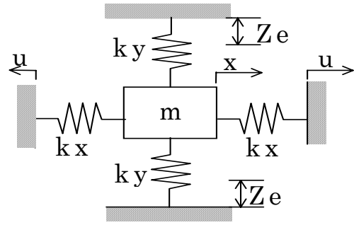
Fig.11 Analytical model
