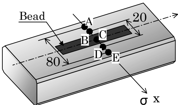
Fig.9 Measuring locations of residual stress of thick plate
